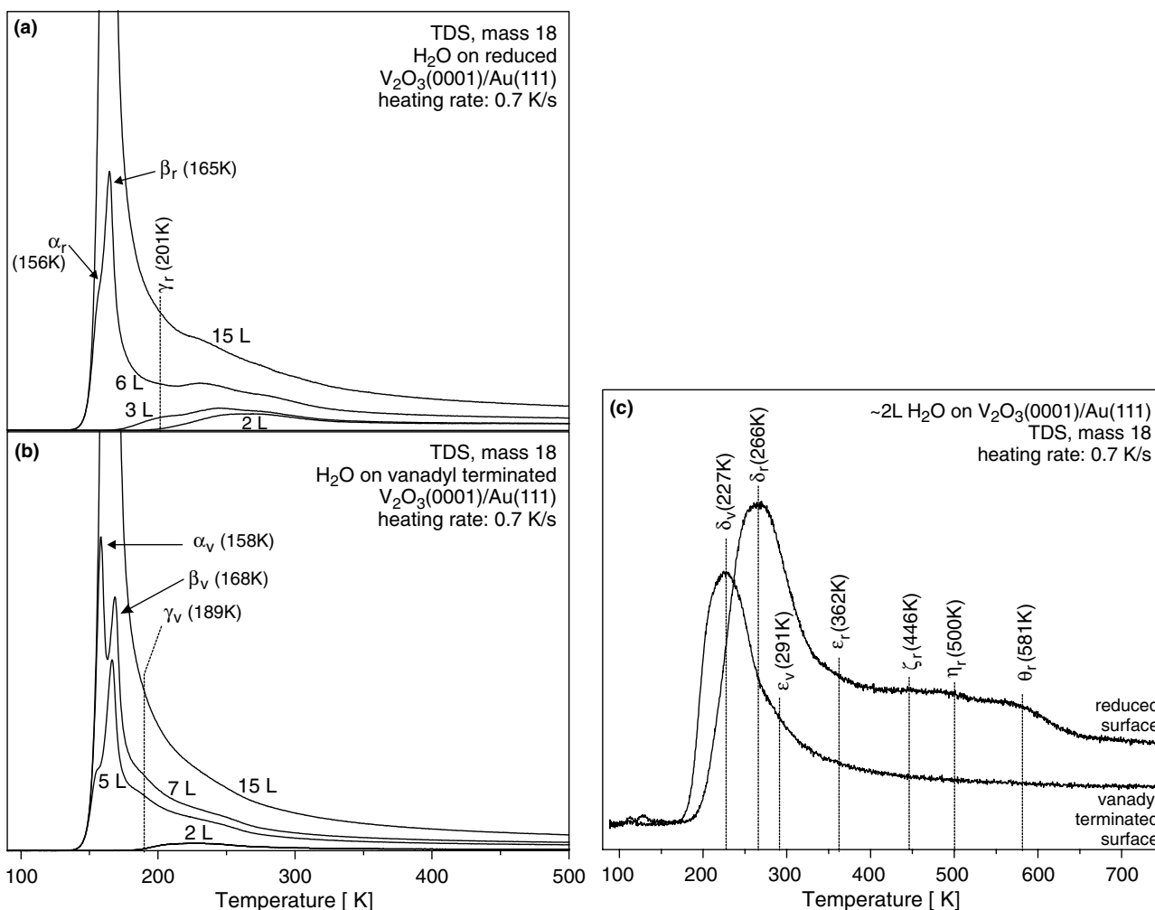
Fig. 6. Left panel: thermal desorption spectra obtained after adsorption of different amounts of water onto reduced (a) and vanadyl terminated (b) V 2 O 3 (0001)/Au(111). Right panel: comparison of the spectra obtained after dosing of 2 L of water on reduced and vanadyl terminated V 2 O 3 (0001) (c). The identified desorption maxima are marked and enumerated by greek letters in the spectra and the desorption temperatures are indicated. The indices 'r' and 'v' refer to the reduced and the vanadyl terminated surface, respectively.
