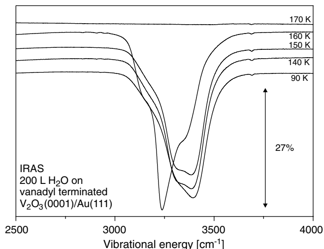
Fig. 5. IRAS data of water on vanadyl terminated V 2 O 3 (0001)/Au(111). Similar to the data shown in Fig. 4(b), but with finer temperature steps near to the multilayer desorption temperature.
