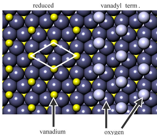
Fig. 1. Structure of the reduced and the vanadyl terminated surface. The surface unit cell is indicated. The structure of the vanadyl terminated surface has been established with STM by Schoiswohl et al. [9]. For the case of the reduced surface unpublished STM data [10] indicate that the surface is terminated by vanadium atoms as shown in the figure.
