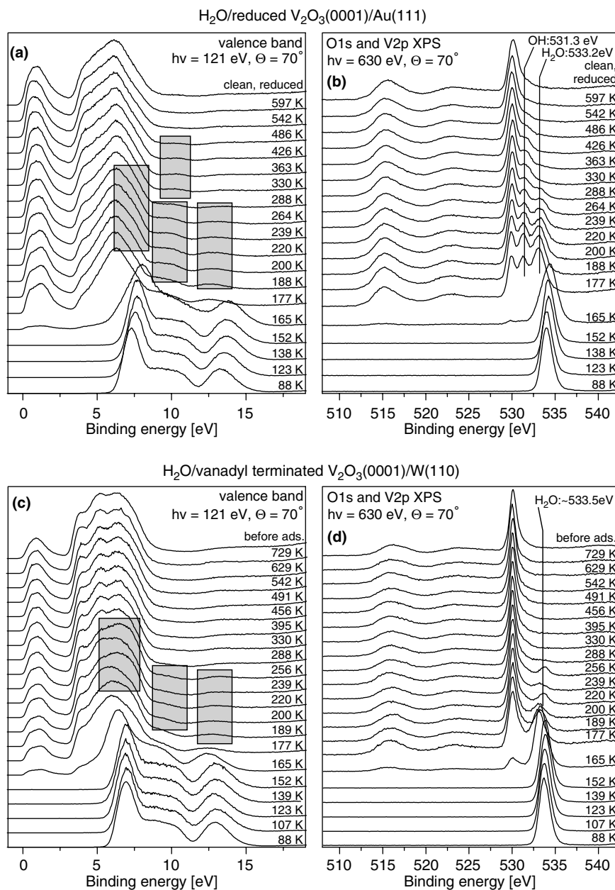
Fig. 3. Photoelectron spectra of the valence band (a,c) and the O1s + V2p region (b,d) of water on vanadyl terminated and reduced V_2O_3(0001) as a function of the annealing temperature. Multilayers of water were adsorbed at 88 K. Before acquiring the spectra for a certain temperature the sample was shortly annealed at this temperature. After this the sample was cooled down and the spectra were recorded at low temperature.
