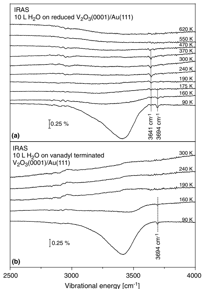
Fig. 4. IRAS spectra of water on reduced (a) and vanadyl terminated (b) V_2O_3(0001)/Au(111) as a function of the annealing temperature. Water was dosed at 90 K and warmed up stepwise. After each annealing step the sample was cooled down again and a spectrum was recorded. We note that there are some features at around 2900\text{ cm}^{-1} and above 3600\text{ cm}^{-1} which are artifacts of the infrared spectrometer. All spectra are referenced to the spectra of the respective non-covered surface, i.e. the spectra shown in panel (a) result from a division of absorption spectra of a water-covered reduced surface by a spectrum of the non-covered reduced surface and the spectra shown in panel (b) result from a division of absorption spectra of a water-covered vanadyl terminated surface by a spectrum of the non-covered vanadyl terminated surface.
