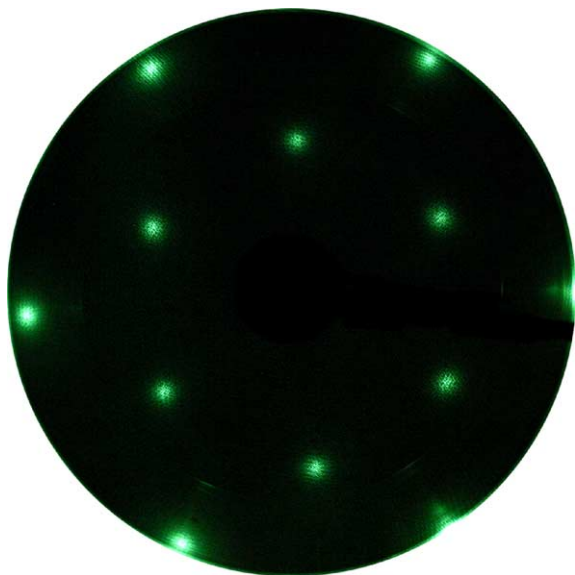
Fig. 2. LEED pattern of V_2O_3(0001)/Au(111) . E_p = 50 eV.
