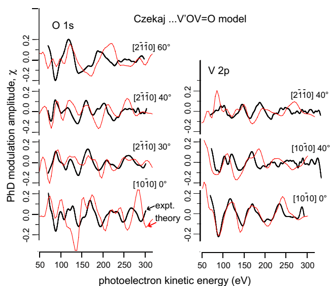
Fig. 3. Comparison of the set of experimental O 1s and V 2p PhD spectra used in this investigation of the V 2 O 3 (0001) surface with the results of multiple-scattering calculations for the vanadyl-covered half-metal termination based on the exact structural parameter values given by total-energy calculations by Czekaj et al.
