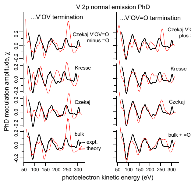
Fig. 4. Comparison of the experimental V 2p normal emission PhD spectrum with the results of multiple-scattering calculations for the half-metal and half-metal-plus-vanadyl oxygen terminations of V_2O_3(0001) using the different sets of interlayer spacings as listed in Table 1.
