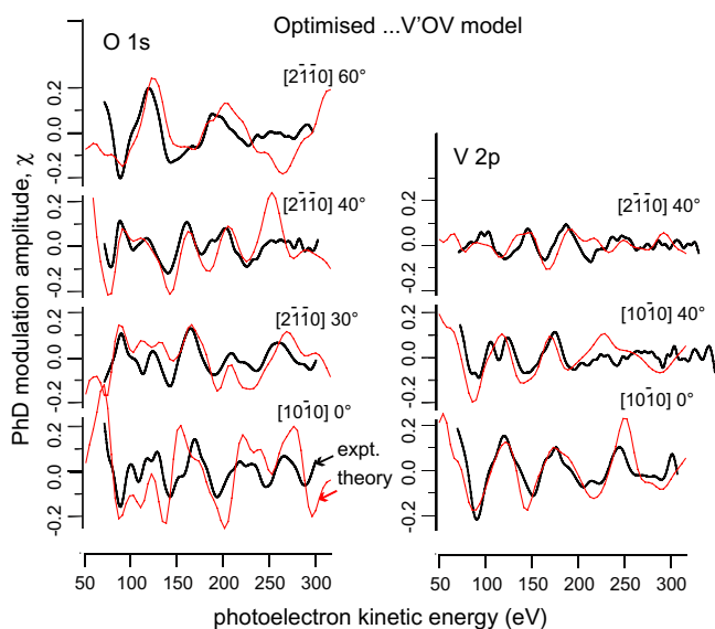
Fig. 5. Comparison of the set of experimental O 1s and V 2p PhD spectra used in this investigation of the V_2O_3(0001) surface with the results of multiple-scattering calculations for the optimised non-vanadyl half-metal termination structure corresponding to the lowest values of the R -factors in Table 2.
