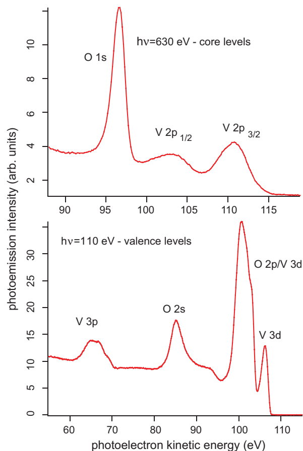
Fig. 2. Typical SXPS spectrum, in the range of the V 2p and O 1s emission peaks, and of the V 3p, O 2s and O 2p/V 3d valence band peaks, recorded from the as-prepared surface of a V_2O_3(0001) epitaxial film grown on Pd(111) at a polar emission angle of 60^\circ .
